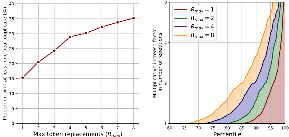
Figure 3: Fuzzy duplicate sequences in The Pile. (a) Proportion of sequences with at least one fuzzy duplicate given the maximum threshold R_{\max} (b) An increase in total number of repetitions if accounting for fuzzy duplicates given the maximum threshold R_{\max} .
